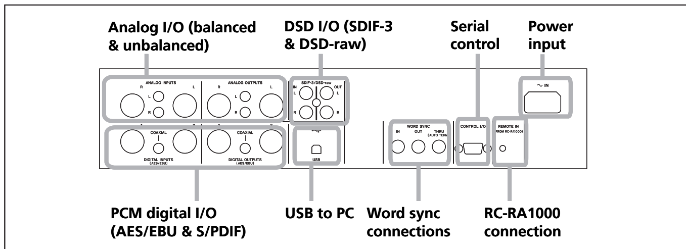
Figure 3.1: Rear panel connections
